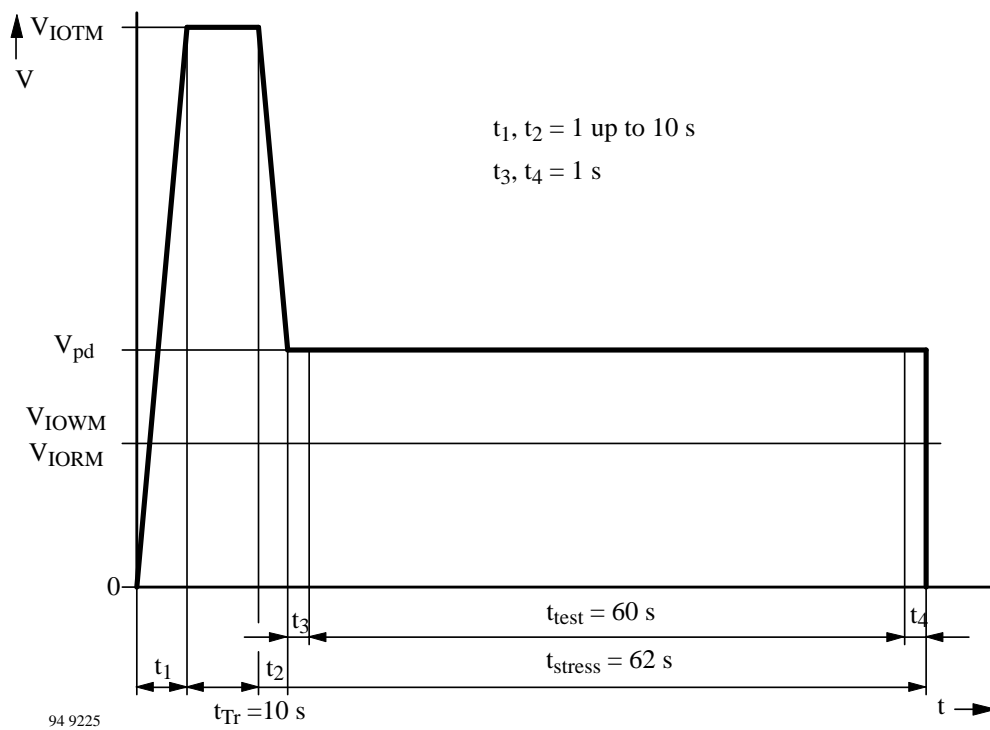
Figure 4. Test pulse for sample test according to DIN VDE 0884
